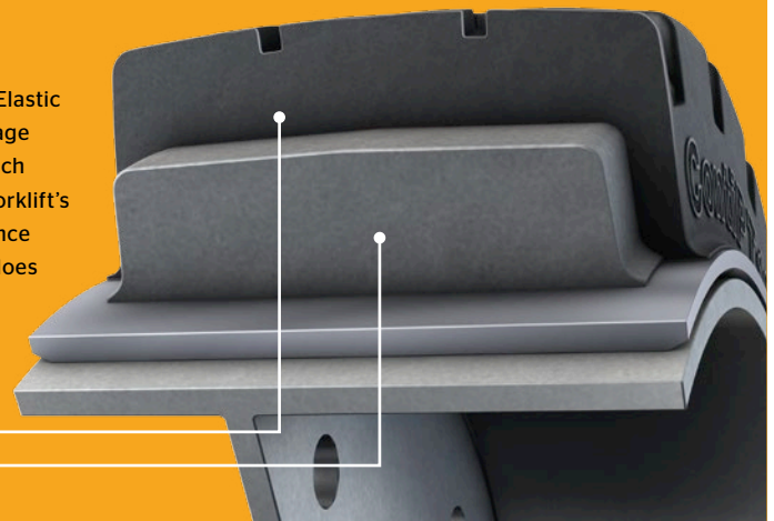
Cut and Tear Resistant Tread Compound Elastic Inner Core
